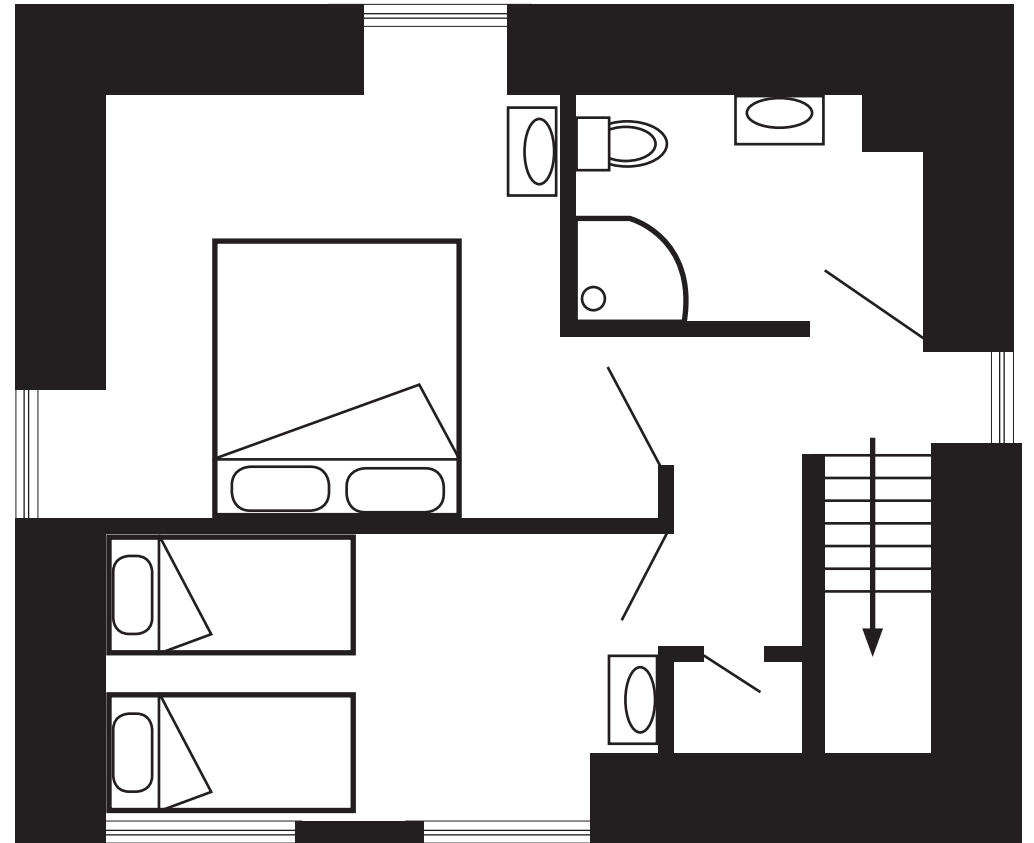
First Floor
